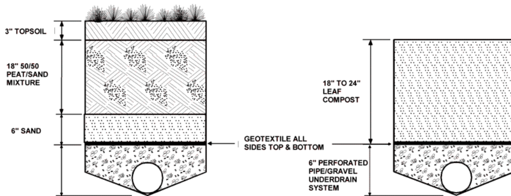
TYPICAL SECTIONS
