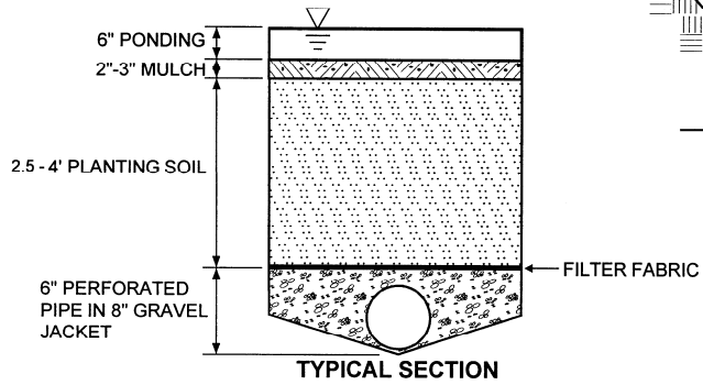
Figure 2.18 Example of Bioretention (F-5)
