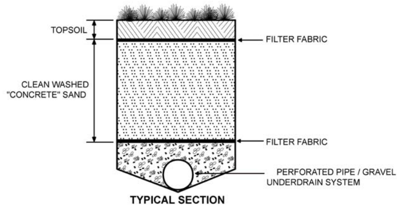
Figure 2.14 Example of Surface Sand Filter (F-1)
